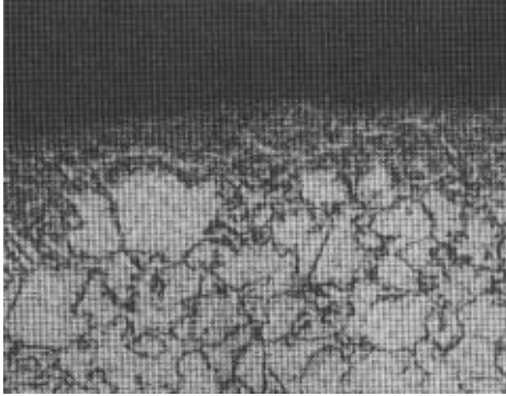
Inter-granular attack due to selective oxidation in 8-gauge wire. (Unetched, X100)
