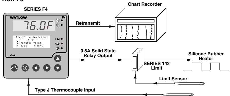
Typical Temperature Controller With SERIES F4 Driving a Chart Recorder
