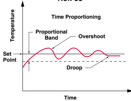
Time vs. Temperature Profile Developed by Proportional Control in a Heat Application
