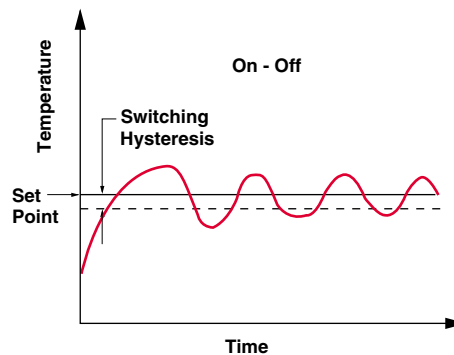
Time vs. Temperature Profile Developed by On-Off Control
