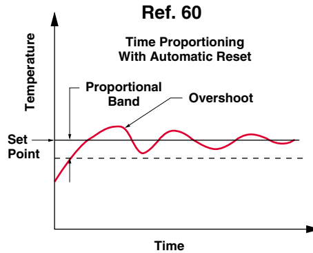
Time vs. Temperature Profile Developed by a Proportional Plus Integral Control in a Heat Application
