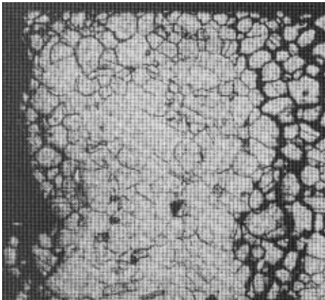
Transverse inter-granular cracks due to sulfur attack in 8-gauge wire. (Electrolytic etch, X35)
