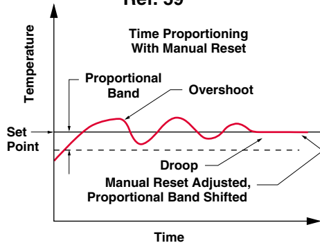
Time vs. Temperature Profile Developed by Proportional Control With Manual Reset in a Heat Application
