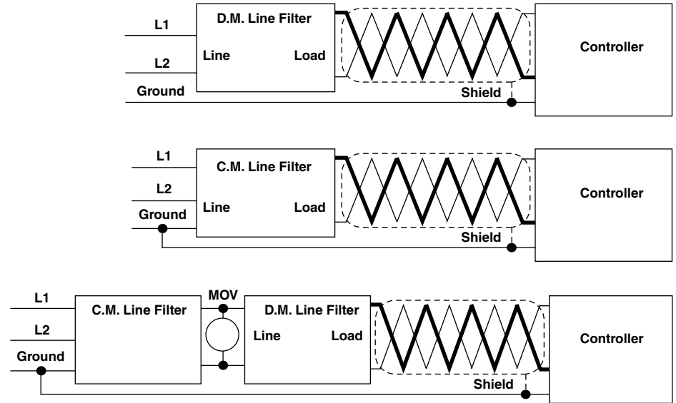
Combination Differential/Common Mode Filter Diagram Ref. 121
